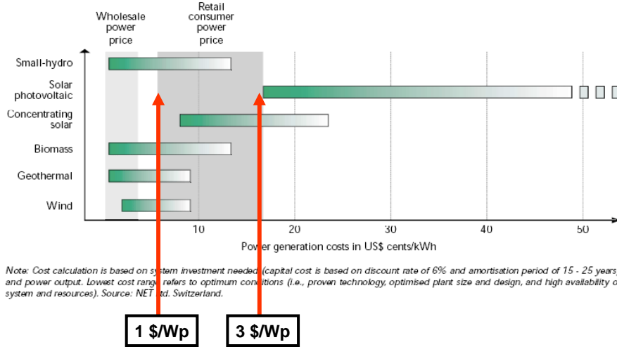
Figure 3-1. Cost Competitiveness of Selected Renewable Power Technologies
